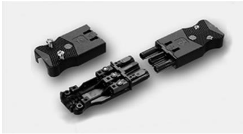
Art. No. MDZ51071ST Stecker | Plug 3-polige | 3-pole ~250V 16A
